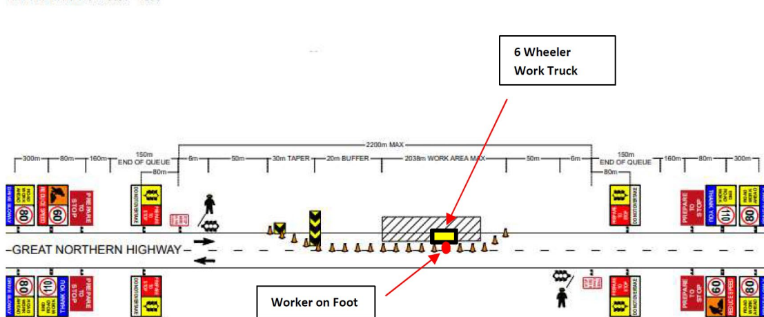
Position of worker on foot and 6-wheeler within traffic management set up.
